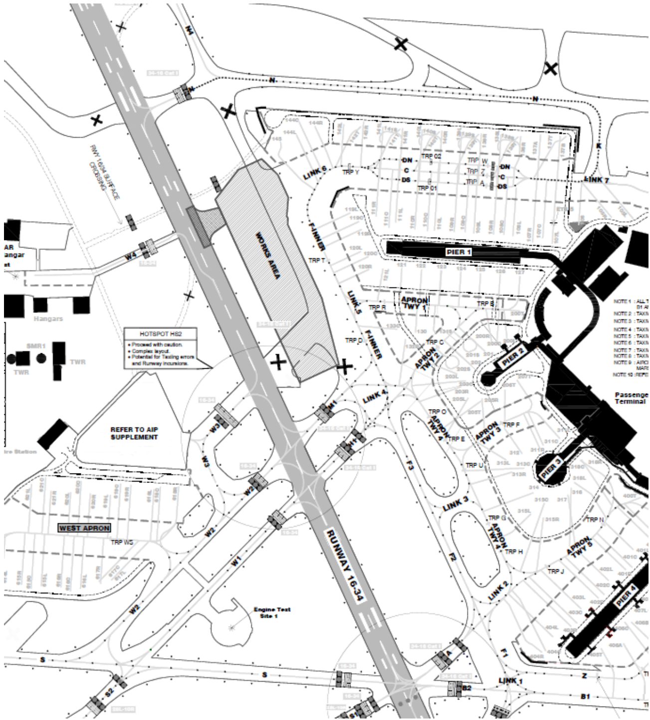
EXTRACT FROM AIP EIDW AD 2.24-2 AIRCRAFT PARKING DOCKING CHART
